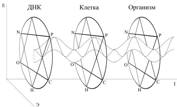
Figure 8. Diagrams of change of the energy-element-informational state of a biological system, coordinates E-Θ-I
