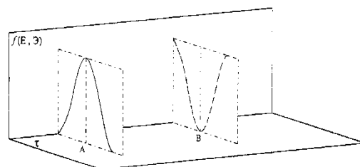
Figure 4: Diagram of dependence of change of the energy-element-informational function f(E, \Theta, I) of biosystem (B) on the change of energy-element-informational function of the Universe (A). Diagram of Le Chatelier-Braun Principle
