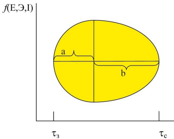
Figure 11. The “Golden Egg” of Life
