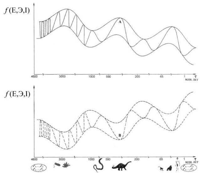
Figure 6. Changing of the function of energy-element-informational state \Delta f(E, \Delta, I) of the Earth (A) and biosystems (B)
