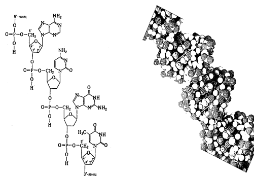
Figure 2: Structural formula and volumetric model of DNA
