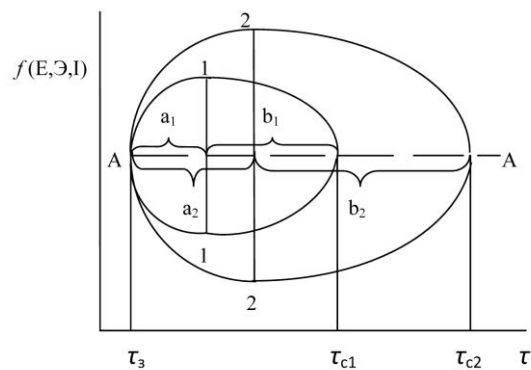
Figure 12. Energy-element-informational model (egg) of life of biosystems 1 and 2; \tau_3 – time of birth (coming into existence), \tau_c – time of death
