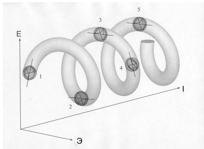
Figure 13. Cyclic change of the function of state f(E, \Theta, I) of the Universe and biosystems 1-5, aligning their equilibrium according to the change of energy-element-informational characteristics of the Universe
