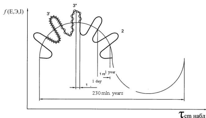
Figure 3. “Dragon of motion”
