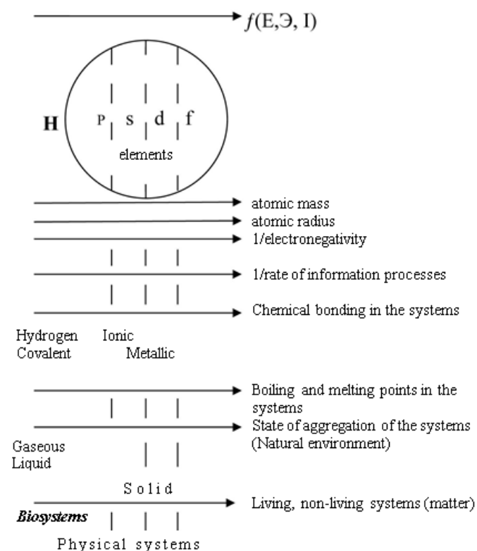
Figure 1 : Energy-element-informational function f(E, \Theta, I) and properties of systems of H, p-, s-, d-, f- elements
