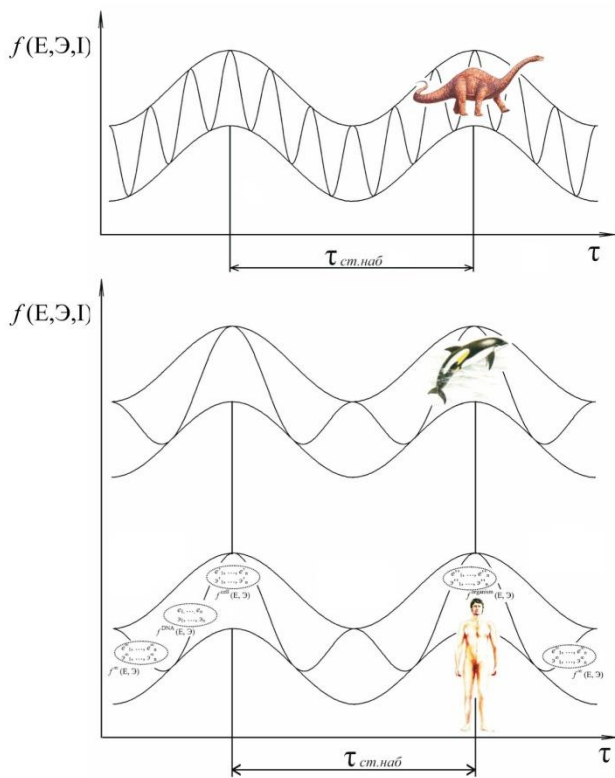
Figure 5 : Organization and development of biological systems (DNA → cell → organism) taking place due to changing of the function of energy-element-informational state \Delta f(E, \Delta, I) of the environment; \tau_{\text{outside observer}} is the length of time reviewed by an outside observer
