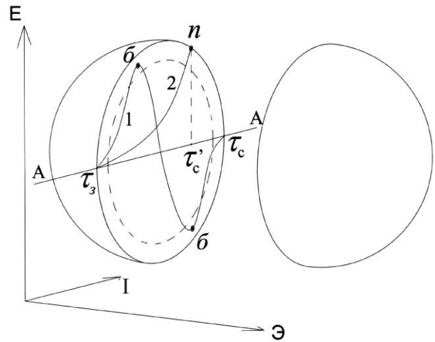
Figure 9 : Model of life of a biological system in the energy-element-informational space; A-A is a line of the energy-element-informational equilibrium; τ is a lifetime of the biosystem from birth (z) to death (c)
