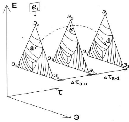
Figure 7 : Diagrams of change of the energy-element state of a physical system, coordinates E-Θ-τ
