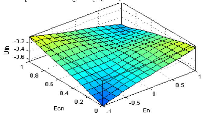
Figure 7. Control surface of FLC controller
