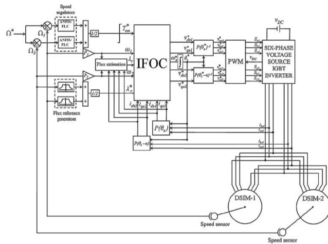
Figure 2. Block diagram of the indirect field oriented control
