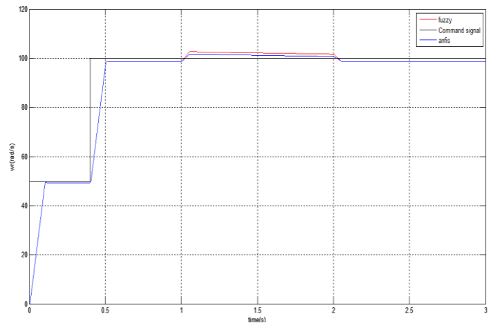
Figure 10. Speed response of DSIM-2
