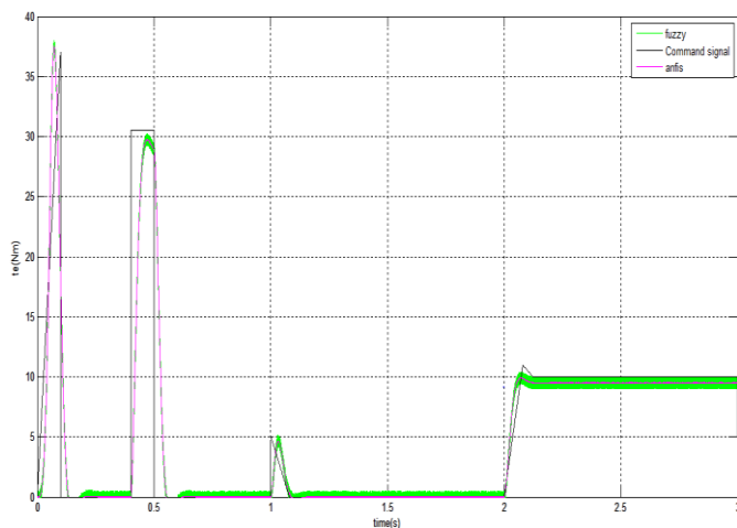
Figure 12. Load response of DSIM-2.
