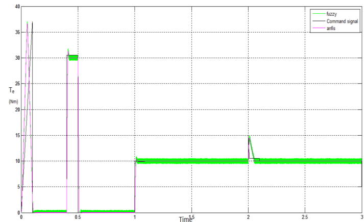
Figure 11. Load response of DSIM-1
