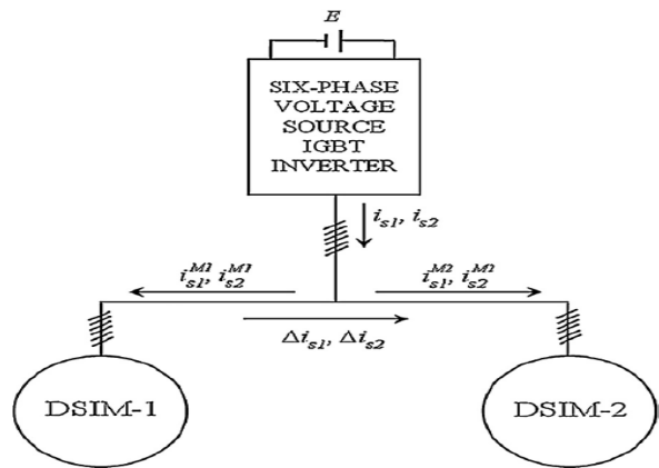
Figure 1. Current flows for parallel connected dual DSIM's.
