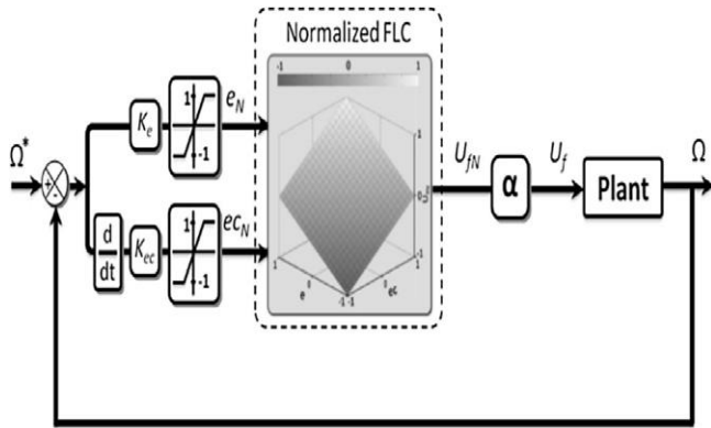
Figure 4. Fuzzy logic controller.
