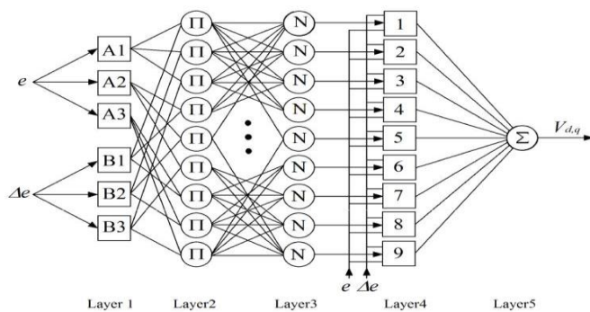
Figure 8. ANFIS structure
