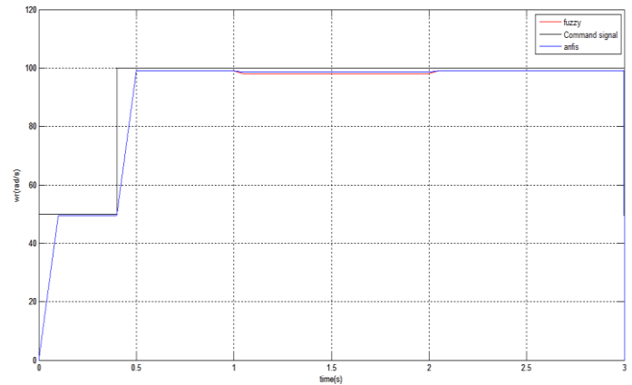
Figure 9. Speed response of DSIM-1
