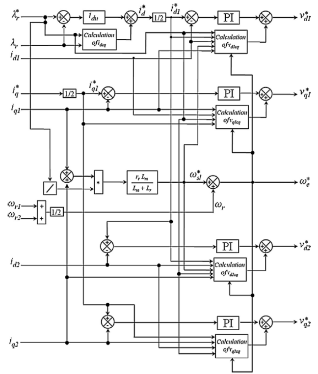
Figure 3. IFOC of the DSIMs.
