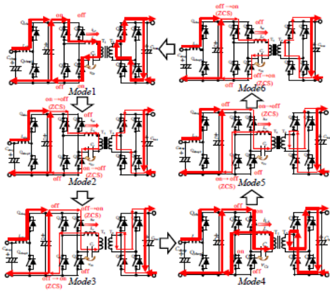
Figure 2. Operation stages for discharge
