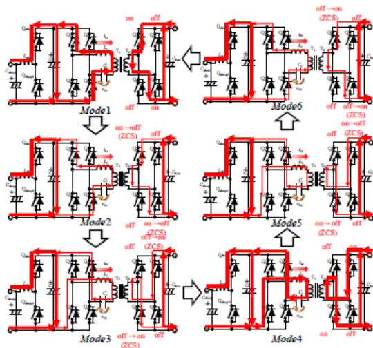
Figure 2. Operation stages for discharge
