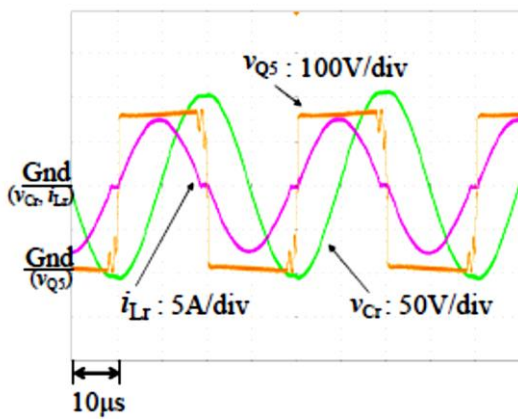
Figure 6. Voltage and current waveform of 10[kW] in the charging
