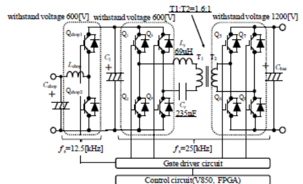
Figure 5. [10kw] circuit structure
