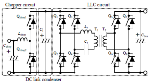
Figure 1. Bi-directional DC-DC converter
