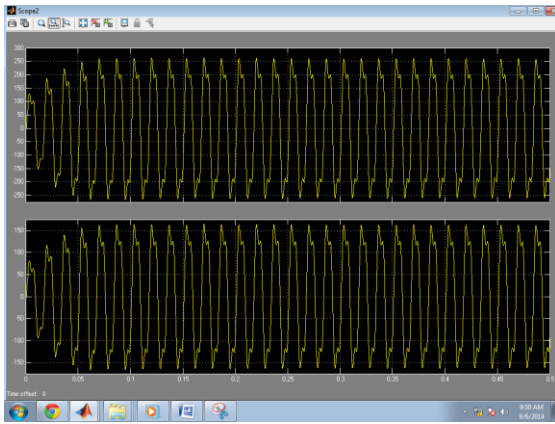
Figure 11. Voltage Versus Time at the Primary and Secondary of the Transformer
