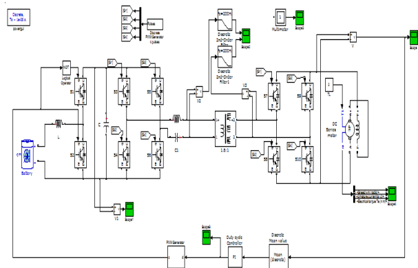
Figure 9. matlab model of 10kw prototype
