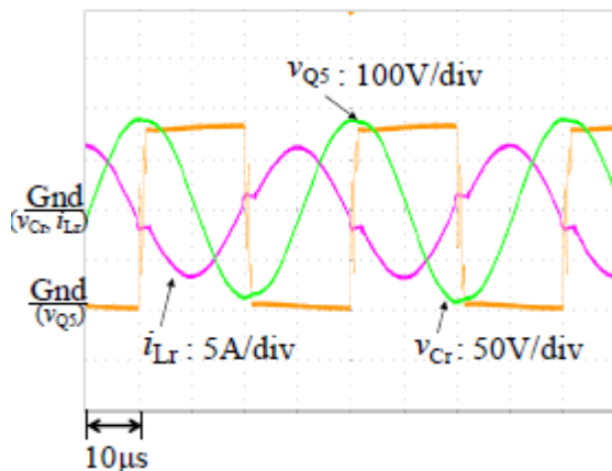
Figure 7. Voltage and current waveform of 6.5[kW] in the discharging
