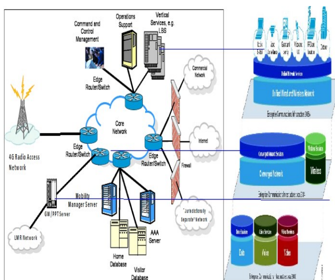
Figure 3.1. Architecture Model of the WSN in the context View
