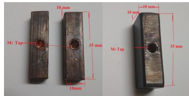
Figure 3. Photographic view of Copper and Tungsten-Copper electrode
