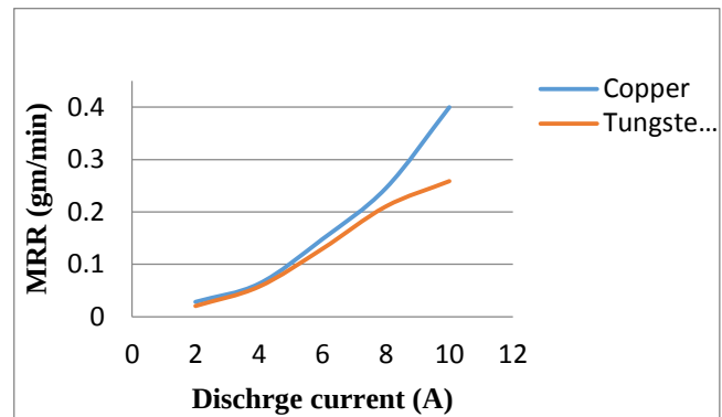
Figure 5. Variation of discharge current verses metal removal rate (MRR) for copper and tungsten copper electrode
