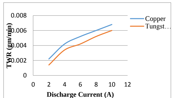
Figure 6. Variation of discharge current verses tool wear rate (TWR) for copper and tungsten copper electrode
