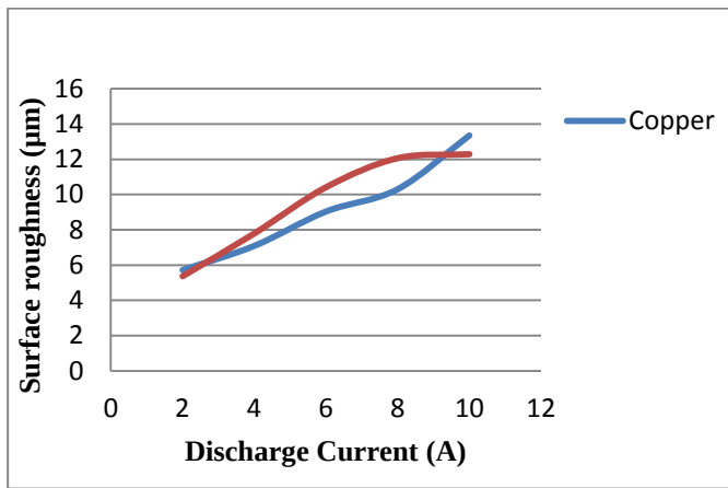
Figure 7. Variation of discharge current verses surface roughness (SR) for copper and tungsten copper electrode
