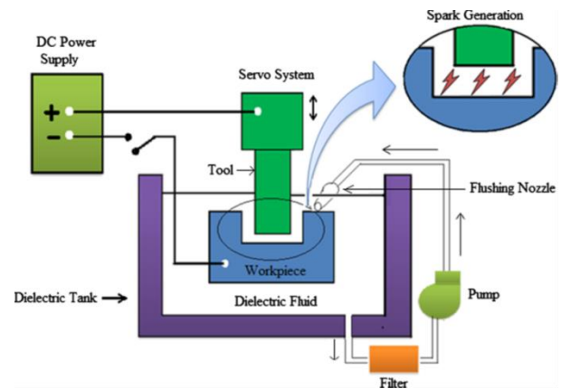
Figure 1. Schematic diagram of experimental set-up for Electro Discharge
