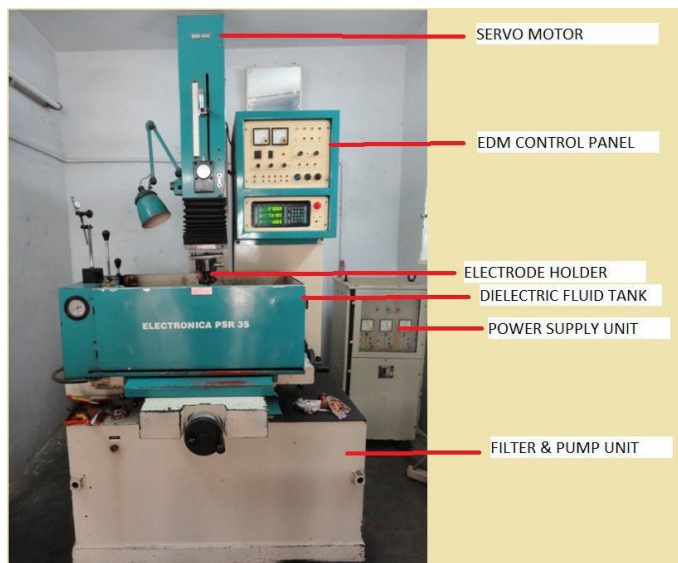
Figure 2. Photographic view of Electro discharge Machine
