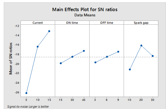
Figure 8. Main effect plot for Sn ratios for MRR
