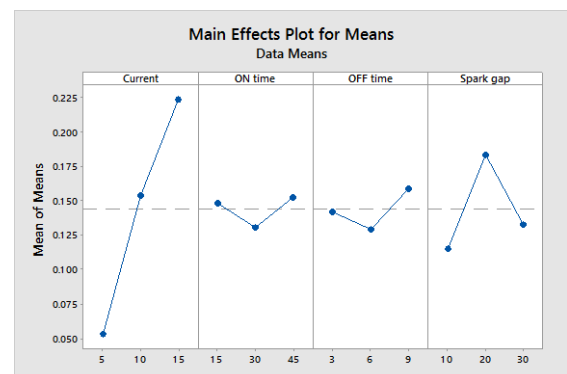
Figure 9. Main effect plots of Means for MRR
