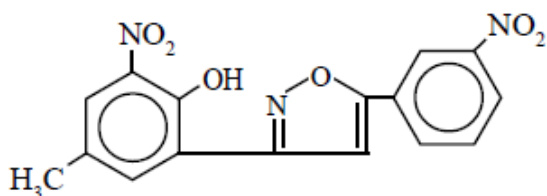
Ligand-III
