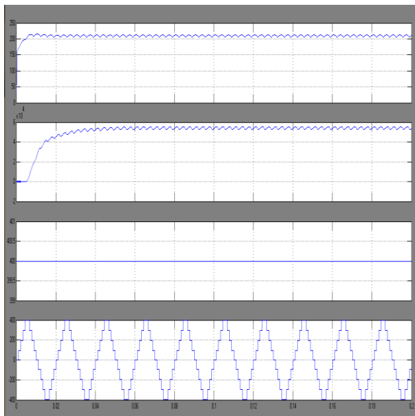
Figure 9. simulation wave form of conventional method PV array dc output, pv power, dc link voltage and inverter voltage
