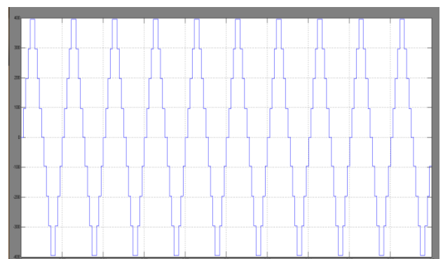
Figure 8. simulation wave form of proposed method of nine- level inverter
