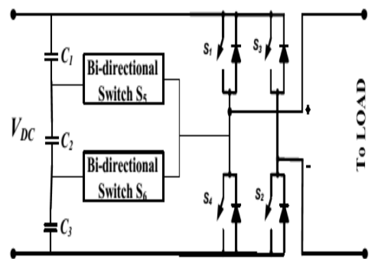
Figure 3. A single phase seven-level Modified PWM Inverter
