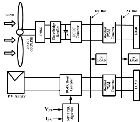
Figure 1. Block diagram of Implemented Hybrid System with Modified PWM converter Topology.
