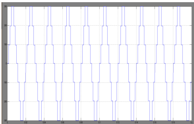
Figure 5. simulation wave form of conventional method seven level inverter
