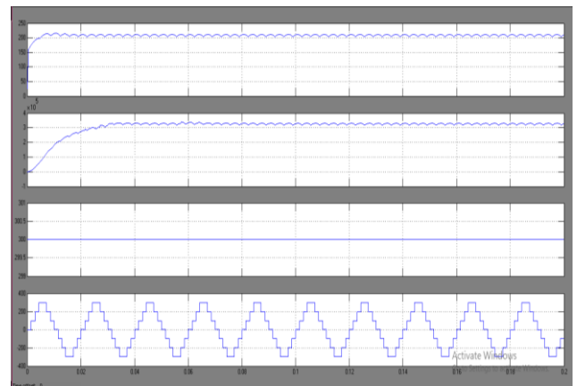
Figure 6. simulation wave form of conventional method PV array dc output, pv power, dc link voltage and inverter voltage
