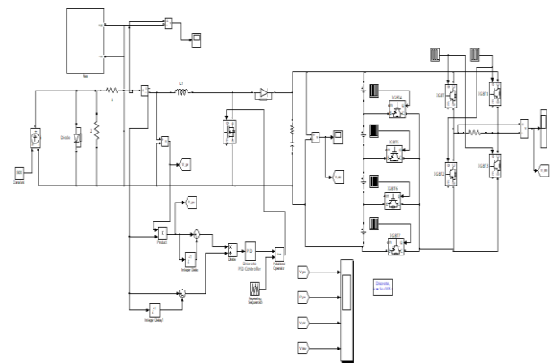
Figure 7. Matlab/Simulink circuit of Implemented Hybrid System with Modified PWM nine level converter Topology.
