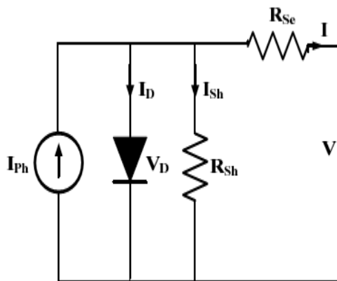
Figure 2. PV (Solar cell) modeling
