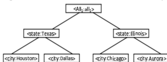
Figure 1. Facet Hierarchy 1
