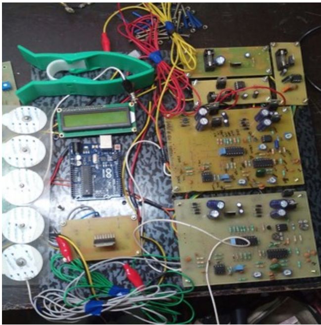
Figure 2. The implemented circuit
