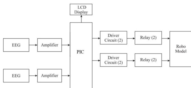
Figure 1. Block Diagram of Brain controlled Wheel Chair
