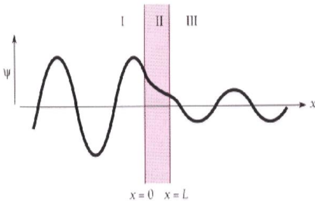
Figure 4. A quantum particle tunneling through a barrier
