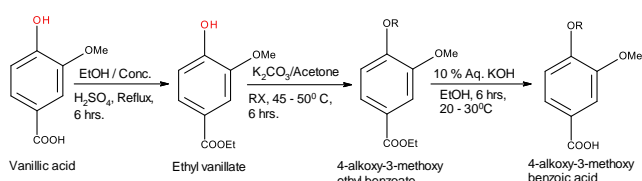
Reaction Scheme 1 :
