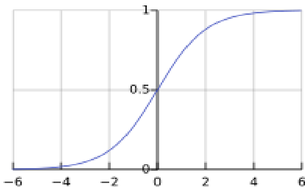
Fig.1.1: Sigmoid function
