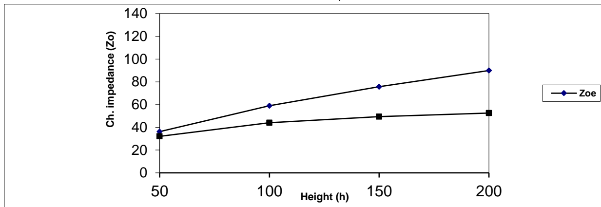
Graph 1: Study of dependence of characteristic impedance on height of the dielectric substrate
