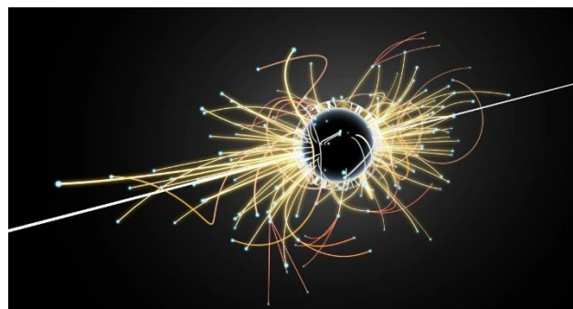
Depicted figure of Self-Interacting Dark Matter particle (SIDM)
