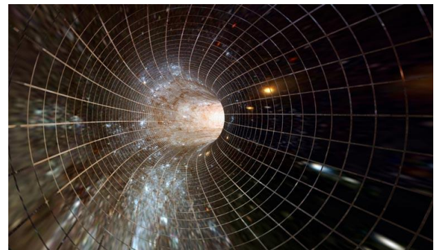
Gravity in Dark Matter
