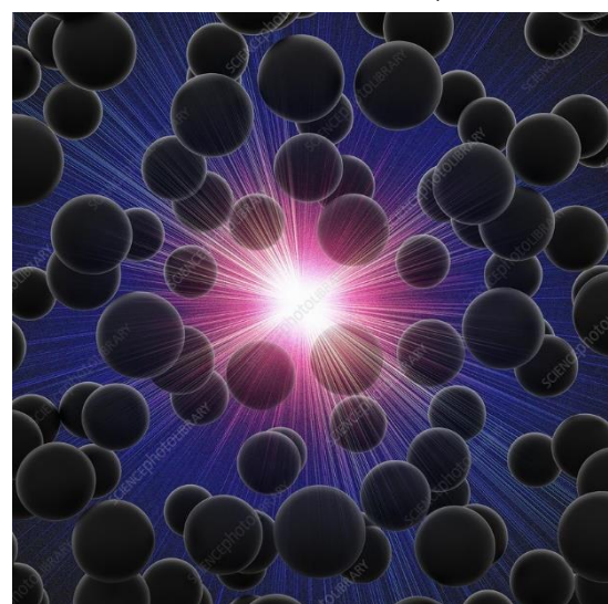
Depicted figure of Strongly Interacting Massive Particles (SIMPs)
