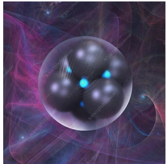
Depicted figure of Stable Massive Particles (SMPs)
