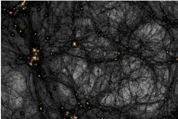
Dark Matter Network
