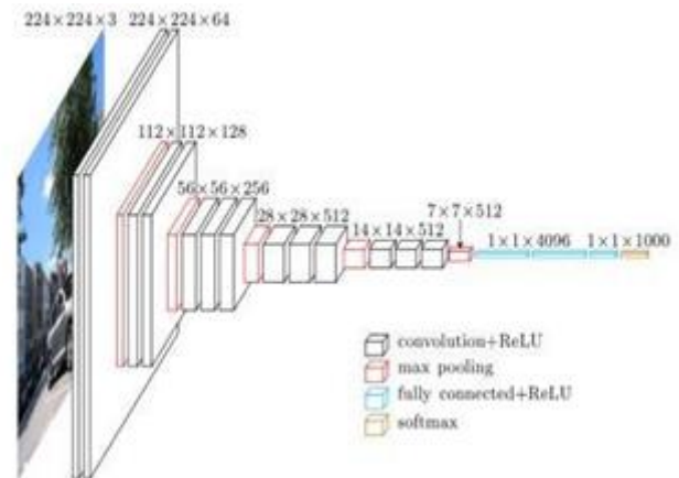
Fig.1 : CNN Architecture
