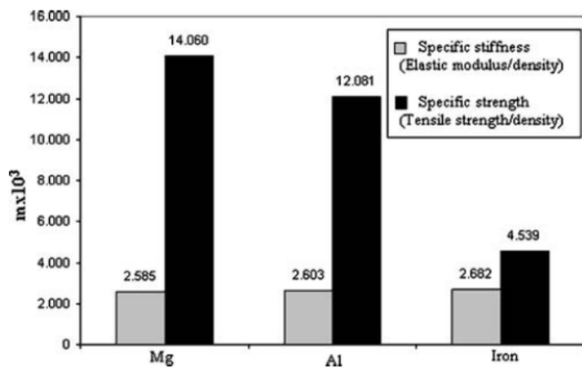
Figure 5. “Comparison of Basic Properties of Mg, Al, and Fe (Mustafa 2008)”(D. S. Kumar et al., 2015).
