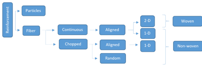
Figure 7. “Types of natural fiber reinforcement, Adapted from(P.K. Mallick, 2007)”.
