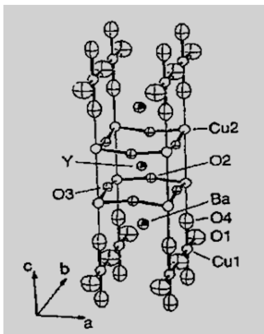
Fig. 1. - Structure of the double-layered YBa_2Cu_3O_7 compound
