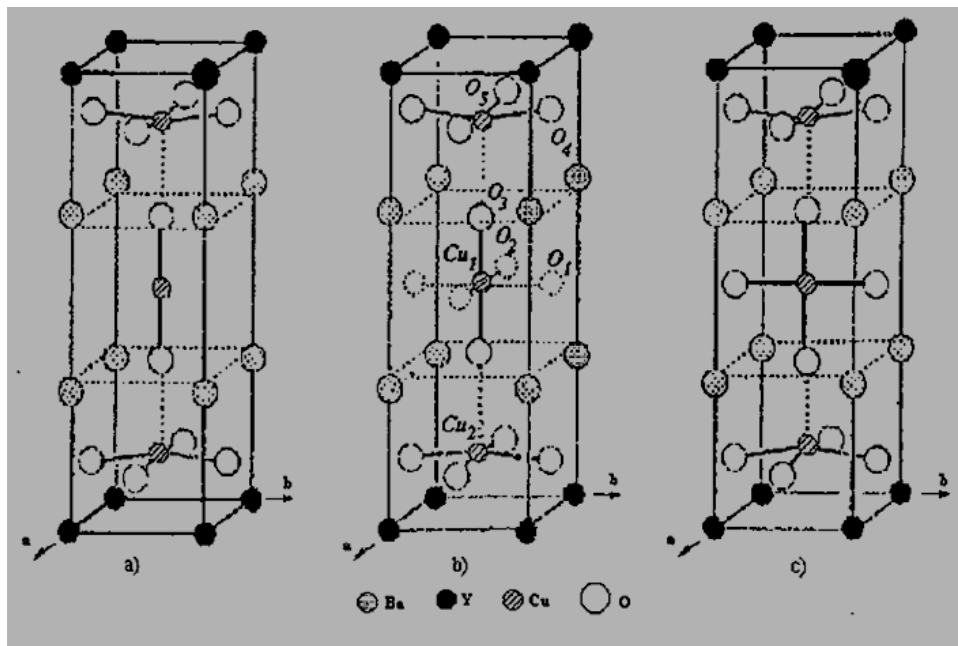
Fig. 3. - The oxygen deficient perovskite structures for YBaCuO system with oxygen content
