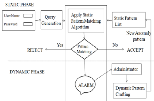
Figure 1.2 Architecture of SQLIA Detection
