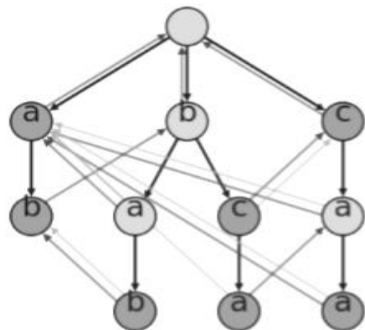
Figure 1.1 Aho–Corasick data structure created from the foreordained word reference
