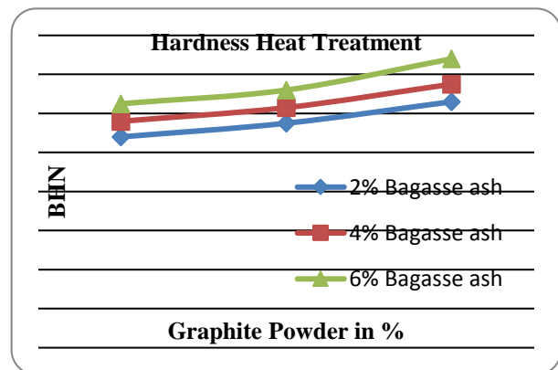
Fig. 13: The effect of Graphite powder and Bagasse ash on the Brinell Hardness of the Heat-treated Hybrid composites at as cast condition.
