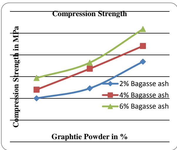
Fig. 12: The effect of Graphite powder and Bagasse ash on the Compression strength of the Heat-treated Hybrid composites at as cast condition.
