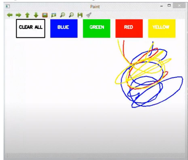
Figure 3: Application GUI.
