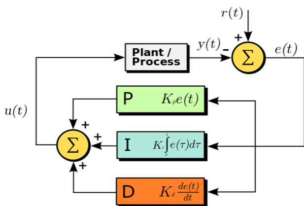
Fig.2 structure of PID
