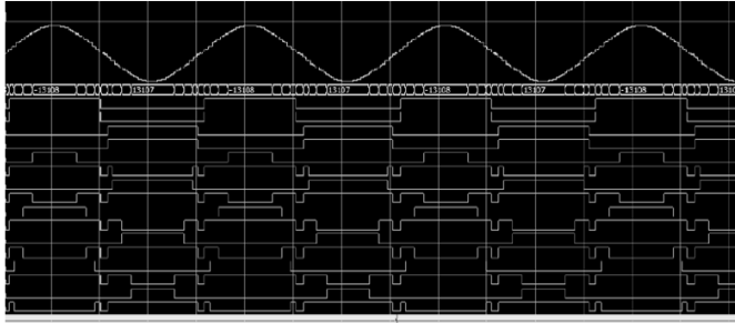
Fig.7. Gate Pulse (V) & Input Voltage (V) waveform of SPWM at rated load
