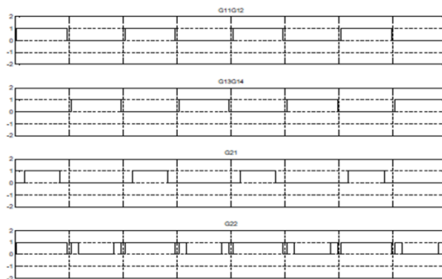
Fig. 5. Sine triangular PWM
