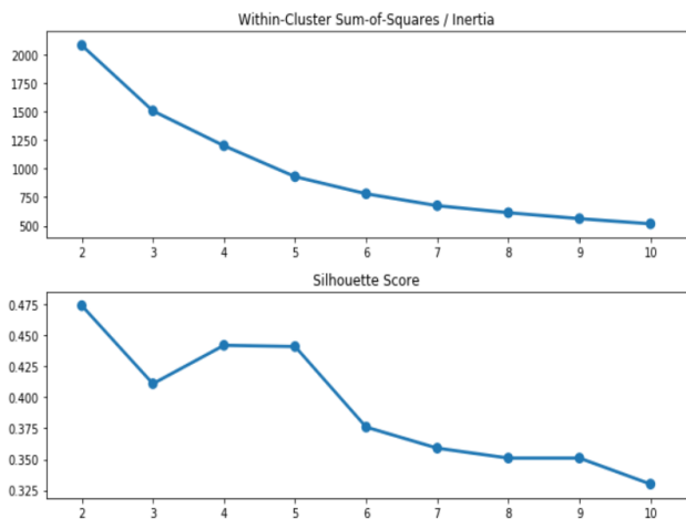
Figure 5 Elbow Graph
