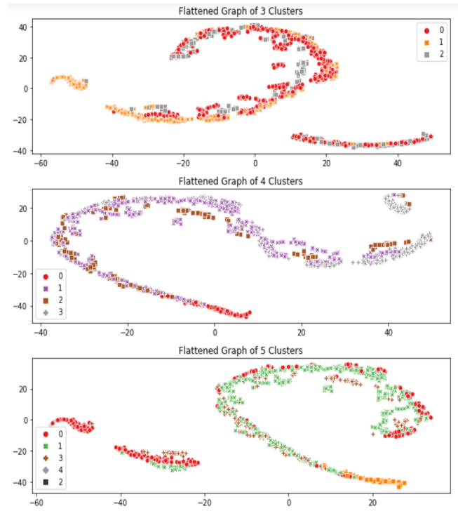
Figure 6 Clustering
