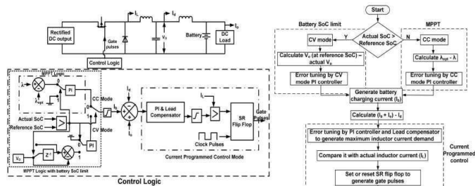
Fig. 2. Block schematic and flowchart of the charge controller circuit for battery
