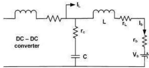
Fig. 3. Circuit representation of buck converter output.
