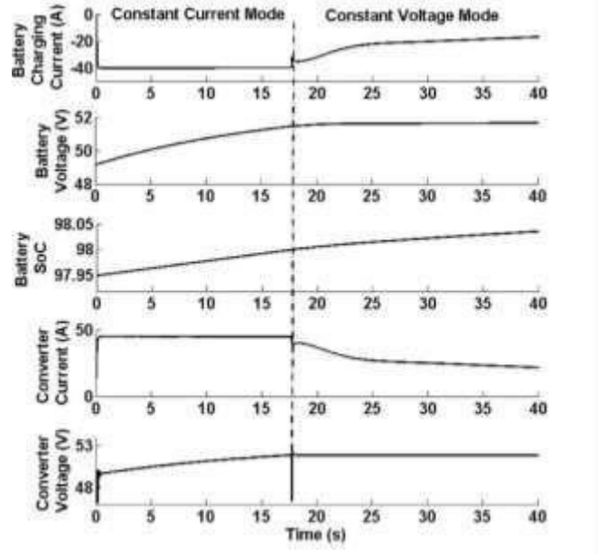
Fig. 5. Battery charging modes at a constant wind speed of 10 m/s.
