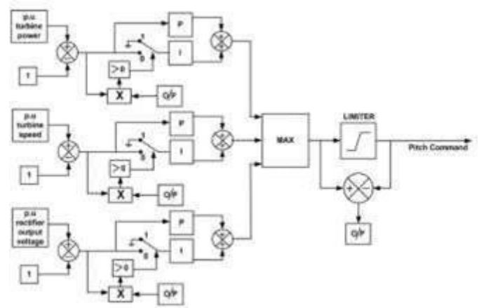
Fig. 7. Pitch control scheme for a stand-alone WECS.
