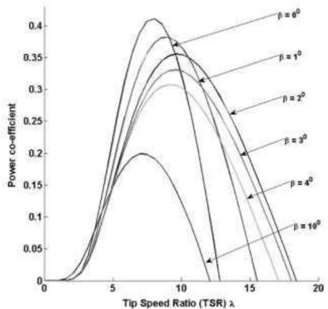
Fig. 6. C_p - \lambda characteristics of the WT for different pitch angles.
