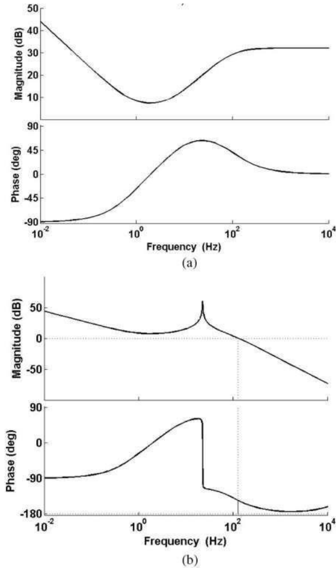
Fig. 4. Bode plot of (a) PI controller in cascade with lead compensator
