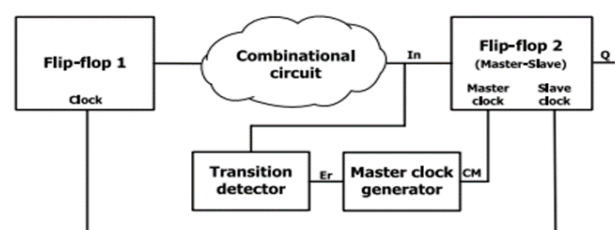
Fig.1: Block diagram of timing error tolerant circuit
