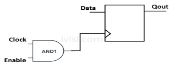
Fig.5: Block diagram of Clock gating
