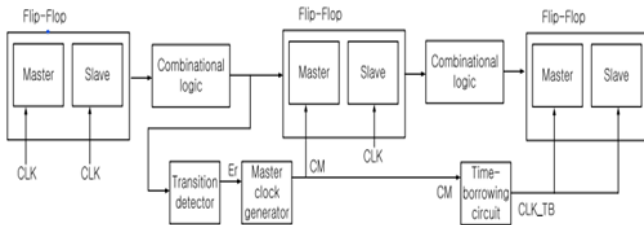
Fig.7: Block diagram of proposed timing error using clock gating.
