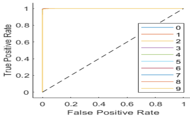
Figure 6: ROC Curve
